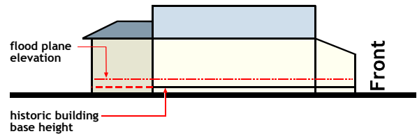
Figure 40 Building Base Height
