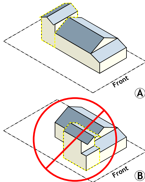
Figure 39 Building Depth
