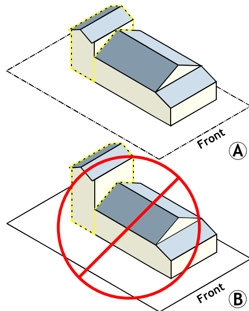
Figure 37 Building Height
