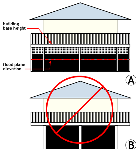
Figure 41 Building Base Height above Flood Level
