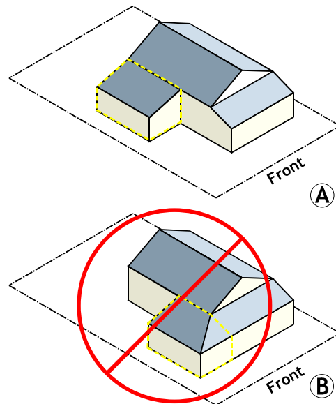
Figure 38 Building Width
